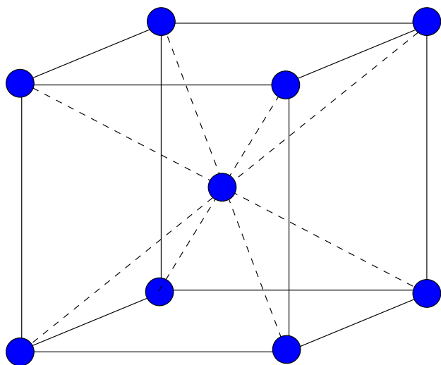
Conventional Cell
