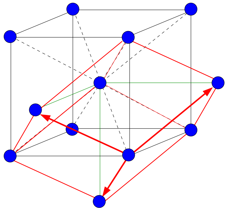
Primitive Cell
